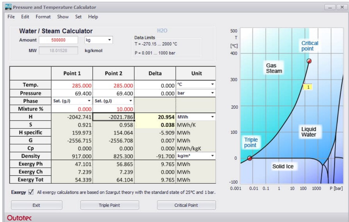
Fig. 3. Evaporation process.
