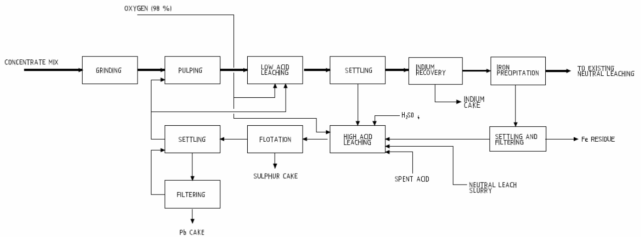
Figure 1. A block diagram of the process implemented for the capacity increase including direct leaching, indium recovery and iron precipitation steps.
