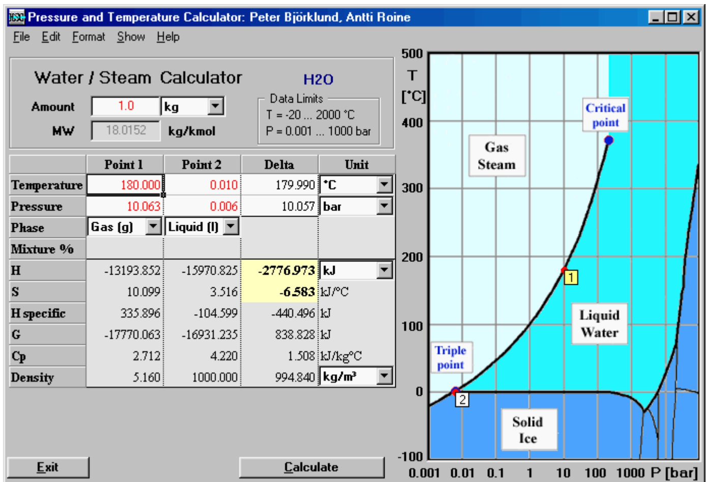
Figure 1: Pressure-Temperature calculator for water.
