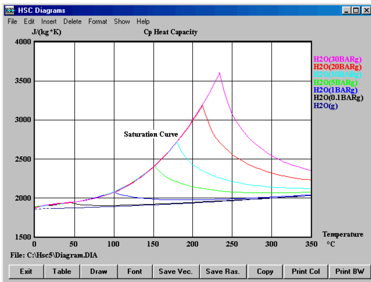
Figure 5: Cp functions for steam at different pressures.
