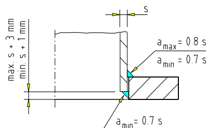
TYPICAL PIPE TO FLANGE WELDING
