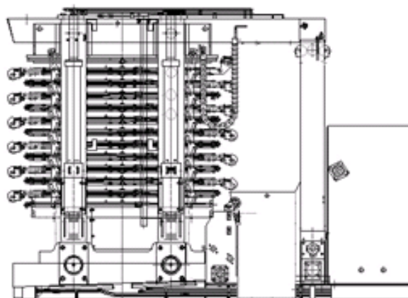
Example: Expanding the PF (12.5/19 m 2 ) with additional filter plates increases the filtration area by 50%.
